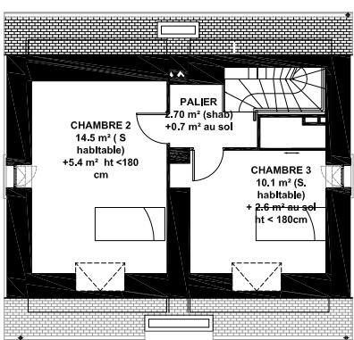
COMBLES
